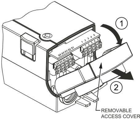
Fig. 9. Access Cover
