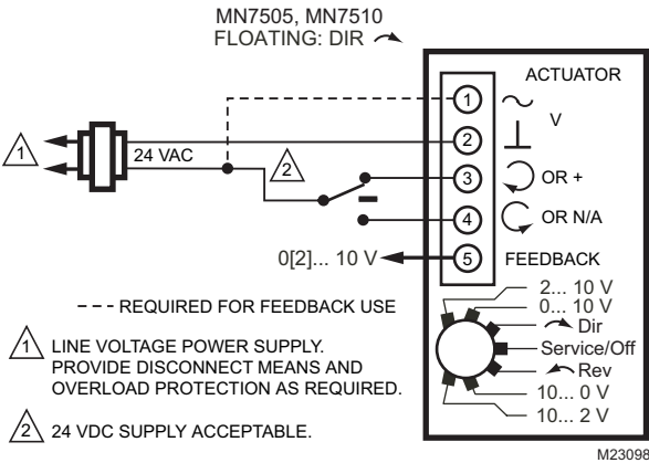
Fig. 11. MN7505/MN7510 (floating mode)
